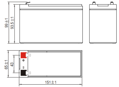
■ T1 Terminal Unit: mm [inches]
