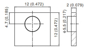
T3 Terminal Unit: mm [inches]
