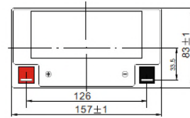
T3 Terminal Unit: mm [inches]
