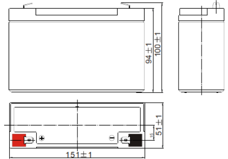
T1 Terminal Unit: mm [inches]
