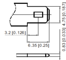
T1 Terminal Unit: mm [inches]
